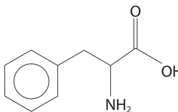
phenylalanine
