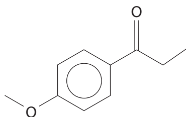
4-methoxypropiophenone
